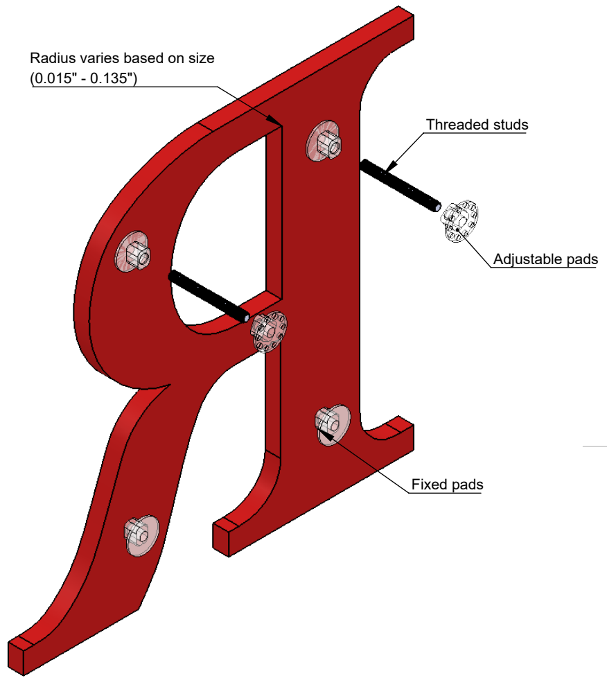
ISOMETRIC VIEW II SCALE 1:3
