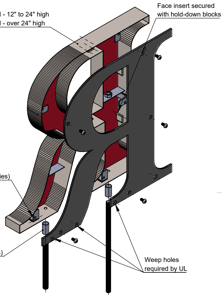
ISOMETRIC BACK VIEW II SCALE 1:4
